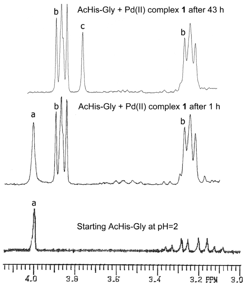
Graphic 1. Parts of ^1\text{H} NMR spectra for the hydrolytic reaction of AcHis-Gly with [\text{HDEA}]_2[\text{PdCl}_4] complex as function of time at pH = 2 and 60^\circ\text{C} in \text{D}_2\text{O} as solvent. The chemical shifts are in ppm relative to TSP. Resonance are indicated as follows: (a) methylene glycine protons of the starting dipeptide; (b) protons of the protonated diethanolamine units of the [\text{HDEA}]_2[\text{PdCl}_4] complex ( 1 ); and (c) methylene protons of the free glycine.
